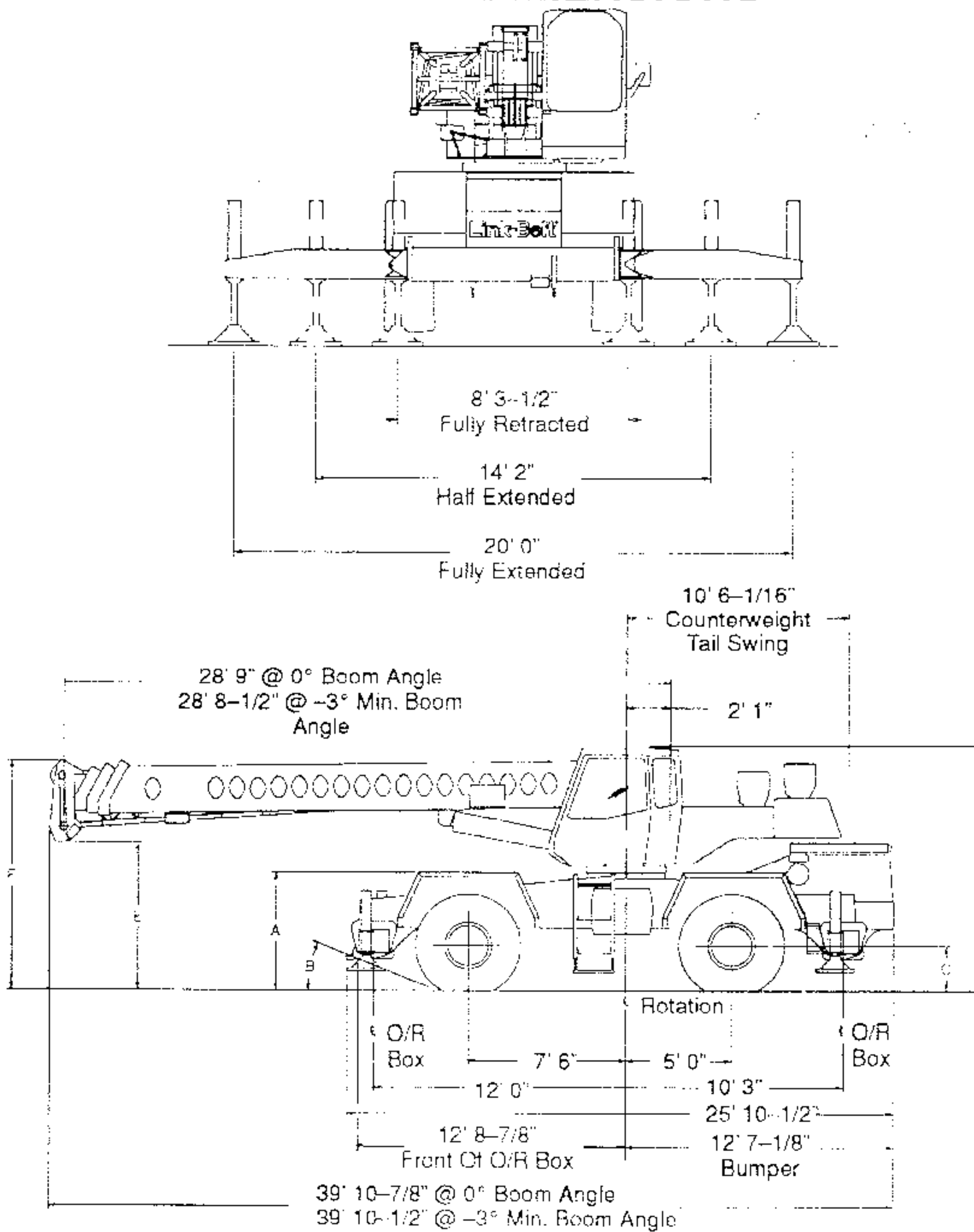
Dimensions Affected By Tires
